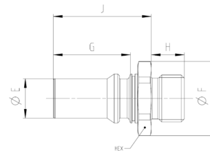
Figure 4 Male ORB ISO 11926-3
