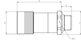
Figure 3 Male BSP
