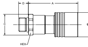
Figure 2 Male ORB
