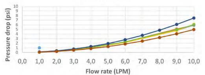
Socket to plug
