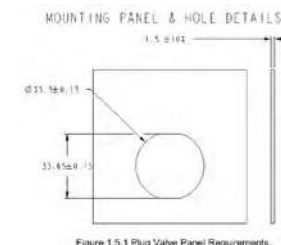
Plug mounting details
